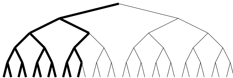
Figure 12.9: Bounded-backtrack search
